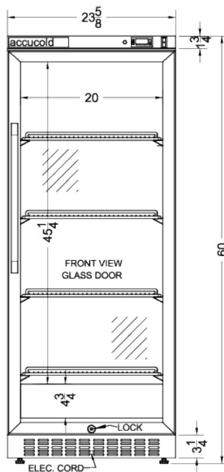
Puretherm Warming Cabinet
