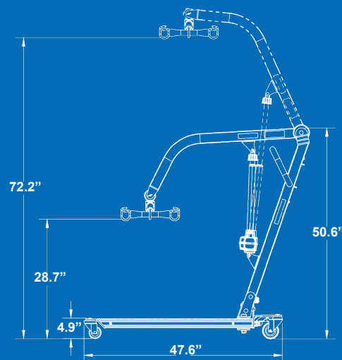
SIDE VIEW OF PL600
