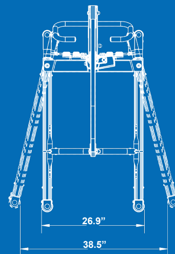
TOP VIEW OF PL600
